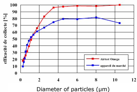
Airtest Omega collection efficiency curve
